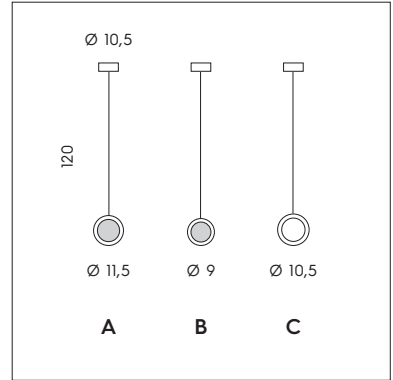
SP 7/330 A - B - C 6W STRIP LED 800 lumen - 3000K CE IP20
